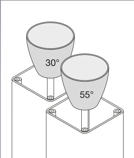
Interchangeable reflectors
