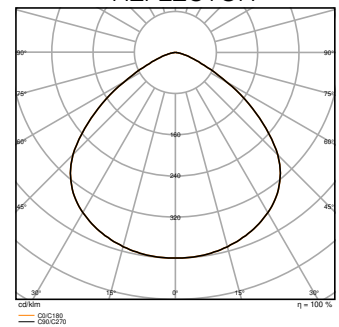
HB P 150W 865 110 DEG IP66 PS set to 125W
