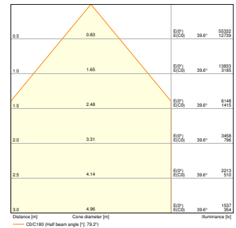
HB P 150W 865 110 DEG IP66 PS - REFLECTOR
