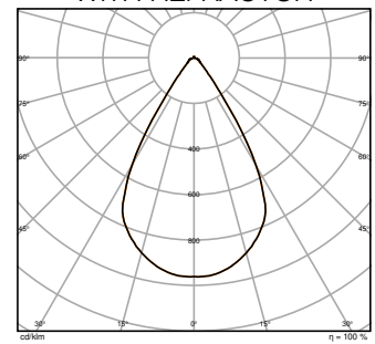
HB DA P 75W 865 70DEG IP66 WITH REFRACTOR
