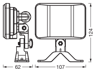
ENDURA FL ADJ 10W 4000K
