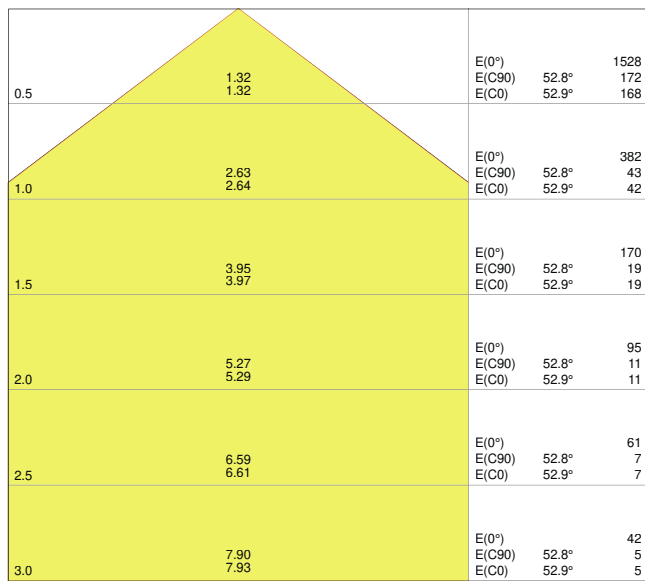
Distance [m] Cone diameter [m] Illuminance [lx] — C0/C180 (Half beam angle [°]: 105.8°) — C90/C270 (Half beam angle [°]: 105.6°)
