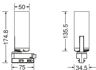
LDPFM Trackspot light 9W
