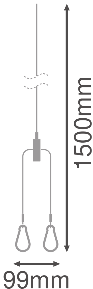
LN SF Suspension Wire
