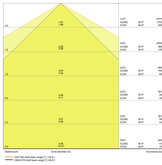
TRUSYS PFM 35W 4000K W DALI
