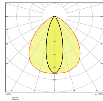
TRUSYS PFM 70W 4000K VN
